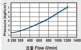
Model: PU520AB-02-S
