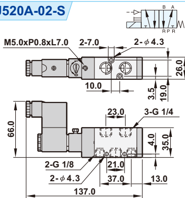
PU520AB-02-S
