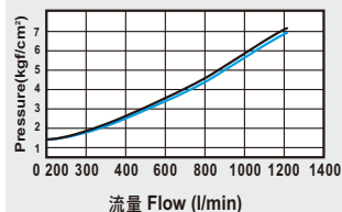
Model: PU520AB-02-S
