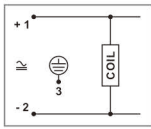
Clamping contact
